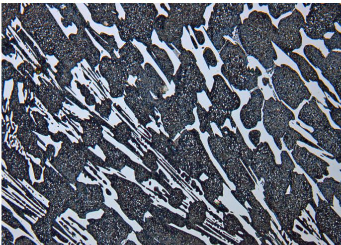
Typical microstructure of 18G alloy (magnification 200X)
