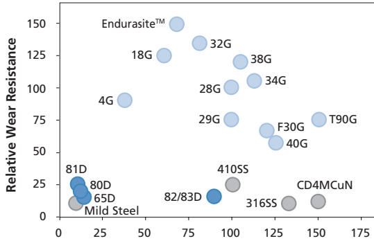
Wear & Corrosion Resistance Index for KSB GIW, Inc. alloys
