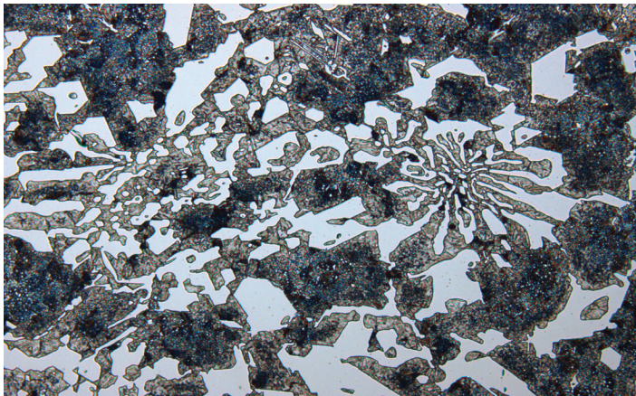
Typical microstructure of 28G alloy (magnification 200X)
